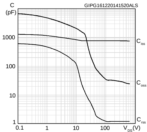
Figure 8: Capacitance variations
