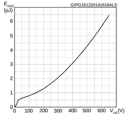
Figure 9: Output capacitance stored energy
