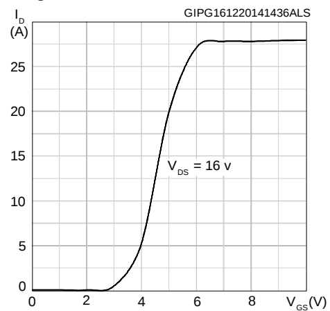
Figure 5: Transfer characteristics
