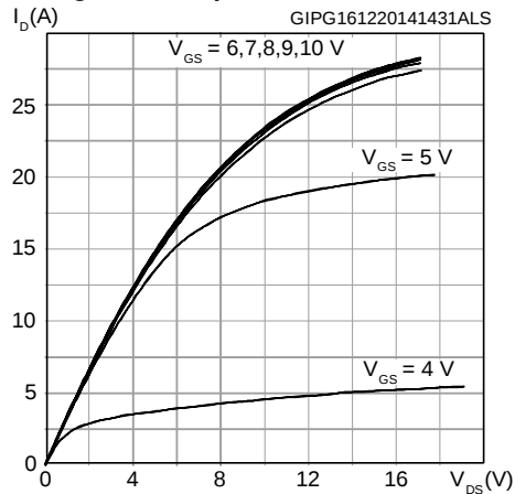
Figure 4: Output characteristics
