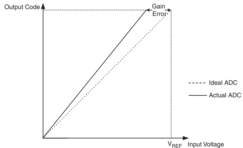
Figure 108. Gain Error
