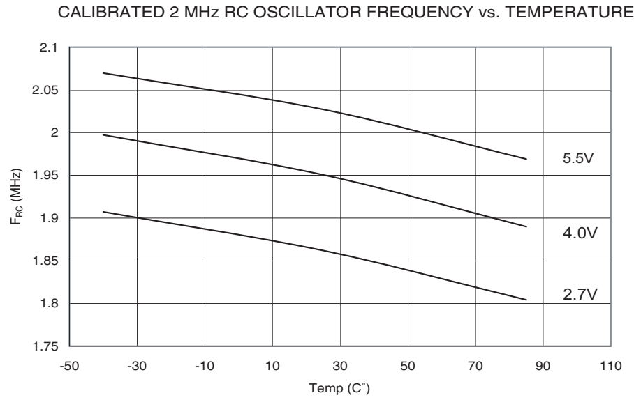
Figure 181. Calibrated 2 MHz RC Oscillator Frequency vs. Temperature
