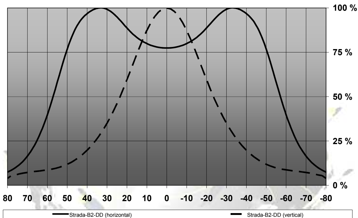
Relative Intensity of C10949_Strada-B2-DD
