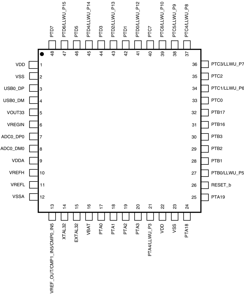
Figure 22. K22 48 LQFP Pinout Diagram
