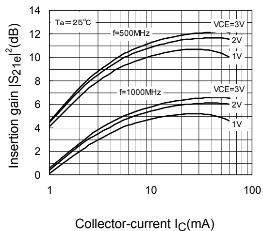
|S_{21e}|^2-I_C
