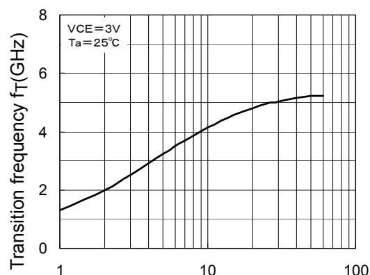
f_T-I_C
