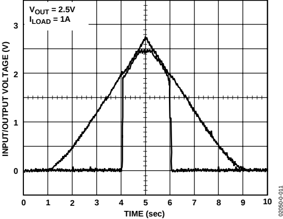
Figure 11. Power-Up/Power-Down
