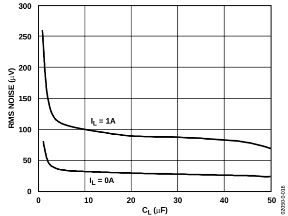
Figure 18. RMS Noise vs. C L (10 Hz to 100 kHz)
