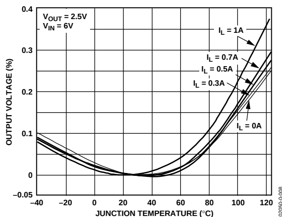
Figure 8. Output Voltage Variation % vs. Junction Temperature
