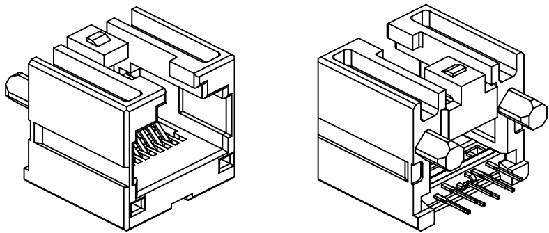
ISOMETRIC VIEWS
