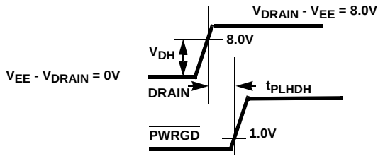
FIGURE 6A. DRAIN HIGH TO \overline{PWRGD} (INACTIVE) HIGH (ISL6142)
