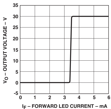
Figure 13. Transfer characteristics.
