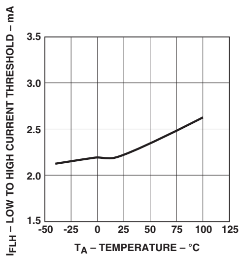
Figure 7. I_{FLH} vs. Temperature.
