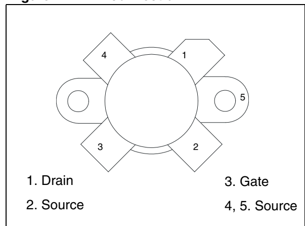
Figure 1. Pin connection
