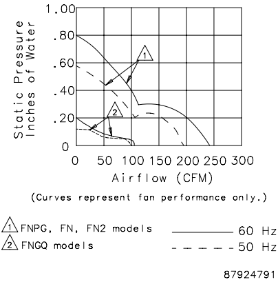
Performance Curve: 6 in. Fans
