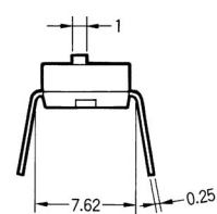
Raised Actuator
