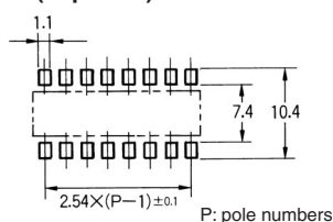
PCB Dimensions (Top View)
