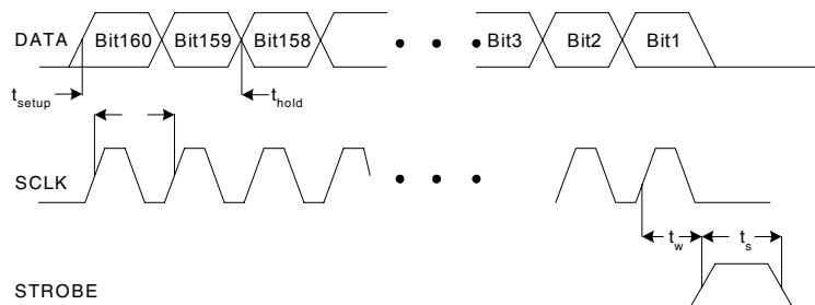
Figure 2. Timing Diagram for Programming the ICS308
