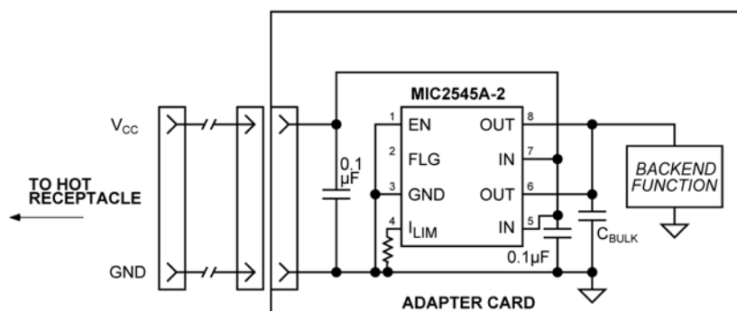
Figure 5. Hot-Plug Application
