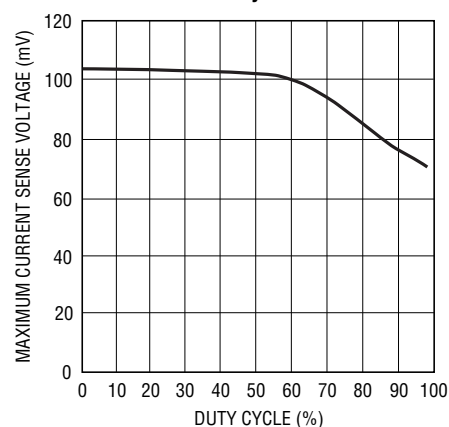
Maximum Current Sense Threshold vs Duty
