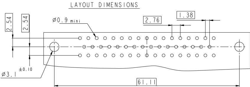
DIMENSION FOR SHELL D WITH METAL BRACKET (50 CONTACTS)
