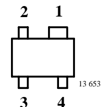
TSDF1250W Marking: WF5 Plastic case (SOT 343) 1 = Collector, 2 = Emitter, 3 = Base, 4 = Emitter
