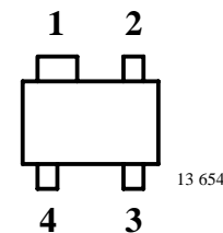
TSDF1250RW Marking: W5F Plastic case (SOT 343R) 1 = Collector, 2 = Emitter, 3 = Base, 4 = Emitter
