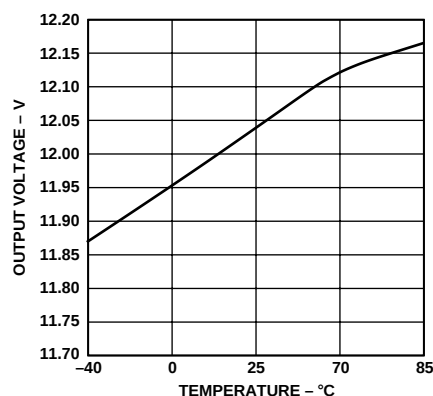
Figure 12. 12 V Output Voltage vs. Temperature
