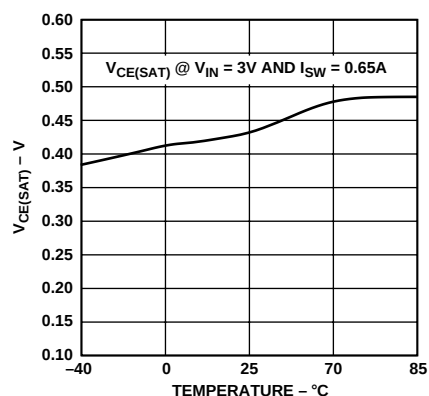
Figure 9. Switch Saturation Voltage vs. Temperature
