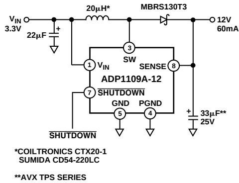
Figure 1. 3.3 V Powered Flash Memory VPP Generator
