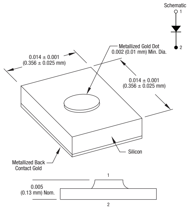
Figure 7. 150-813 Package
