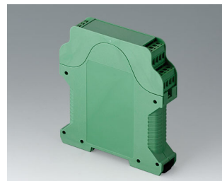
B6721721 RAILTEC CV WIDTH 0.886", without ventilation slots PA 6 (UL 94 V-0) green 0.89"x4.41"x3.90"
