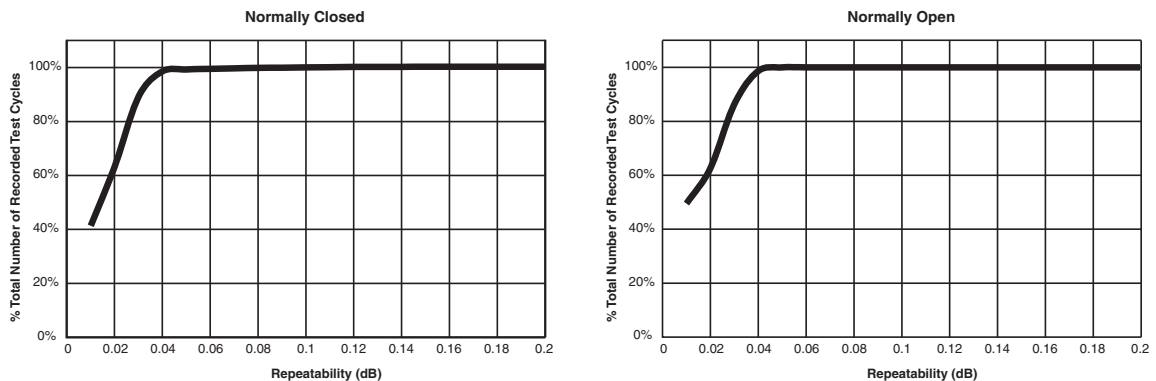
REPEATABILITY CHARACTERISTICS GRF303 RELAYS
