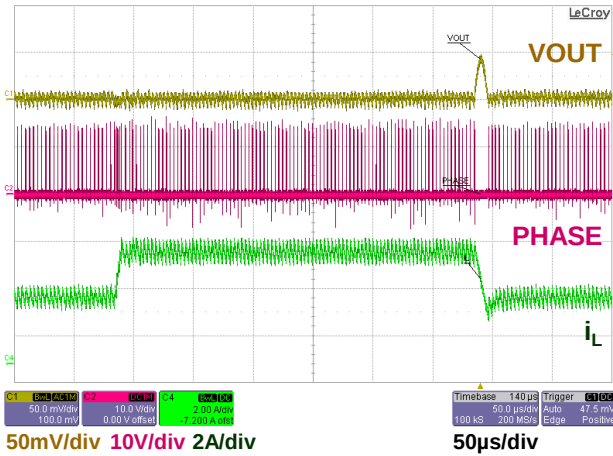
Figure 15: Load Transient 3-5A
