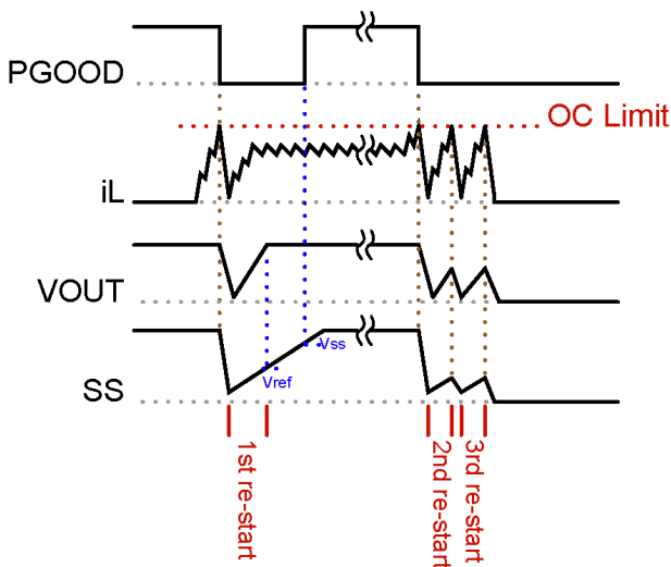
Figure 23. Over Current Protection
