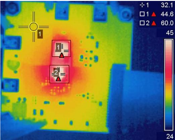
Figure 18: Thermal Image at VIN = 12V, IOUT = 6A (IR3863: 60°C, Inductor: 45°C, PCB: 32°C)
