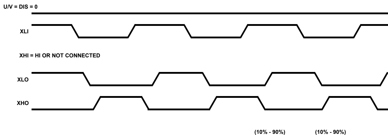
FIGURE 2. BISTATE MODE
