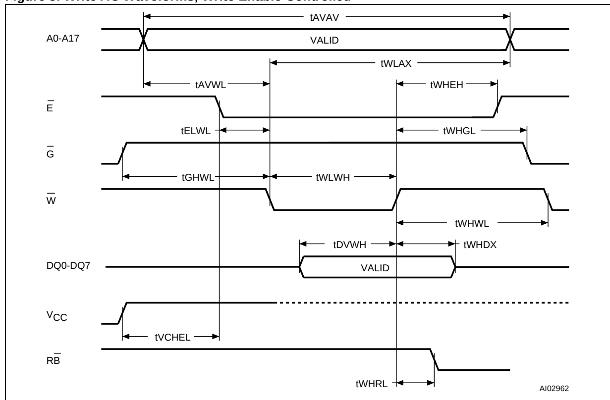
Figure 8. Write AC Waveforms, Write Enable Controlled
