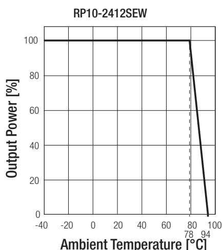
Derating Graph (11)
