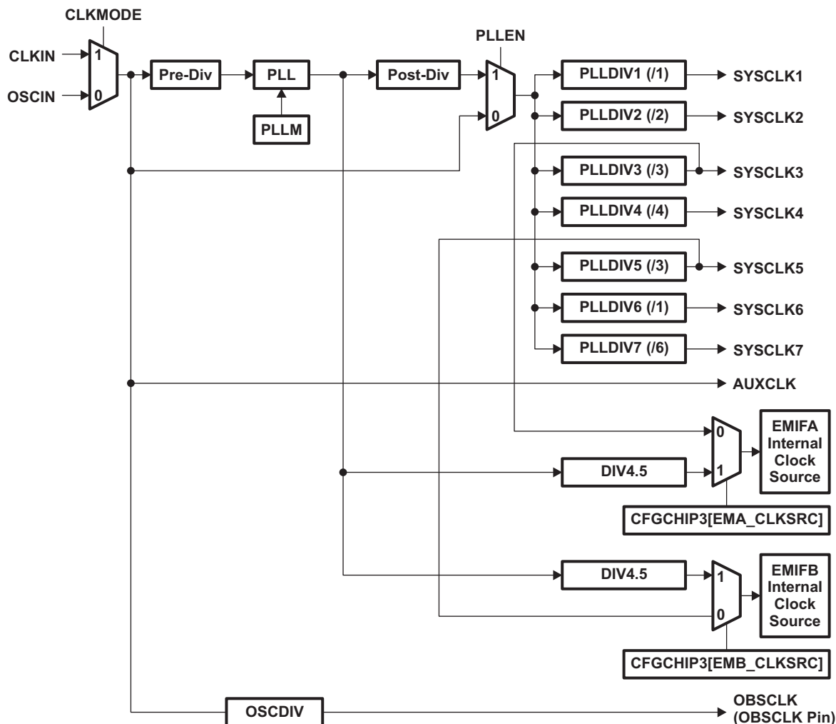
Figure 6-9. PLL Topology
