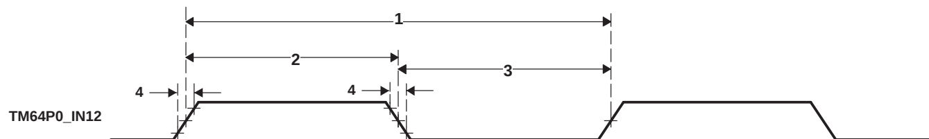
Figure 6-60. Timer Timing
