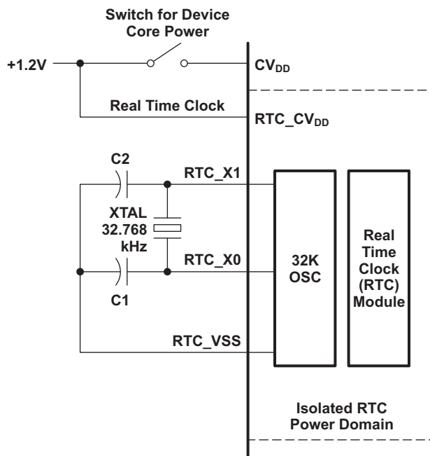
Figure 6-74. Clock Source
