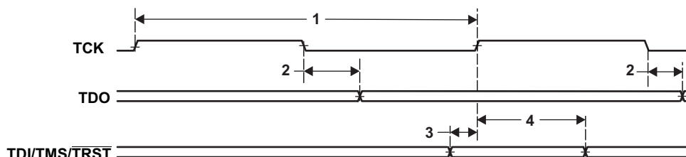
Figure 6-72. JTAG Test-Port Timing
