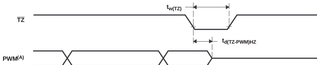
Figure 6-46. PWM Hi-Z Characteristics
