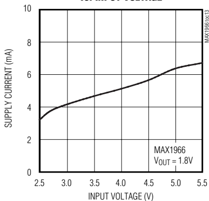
MAX1966 SUPPLY CURRENT vs. INPUT VOLTAGE
