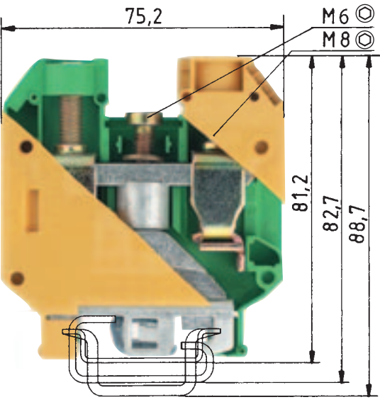
closed design
