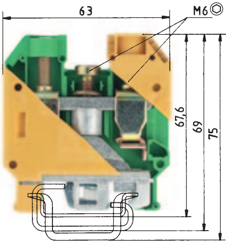
closed design
