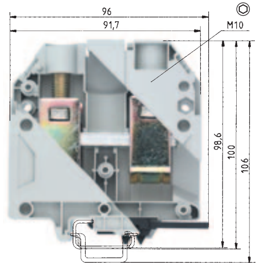
closed design
