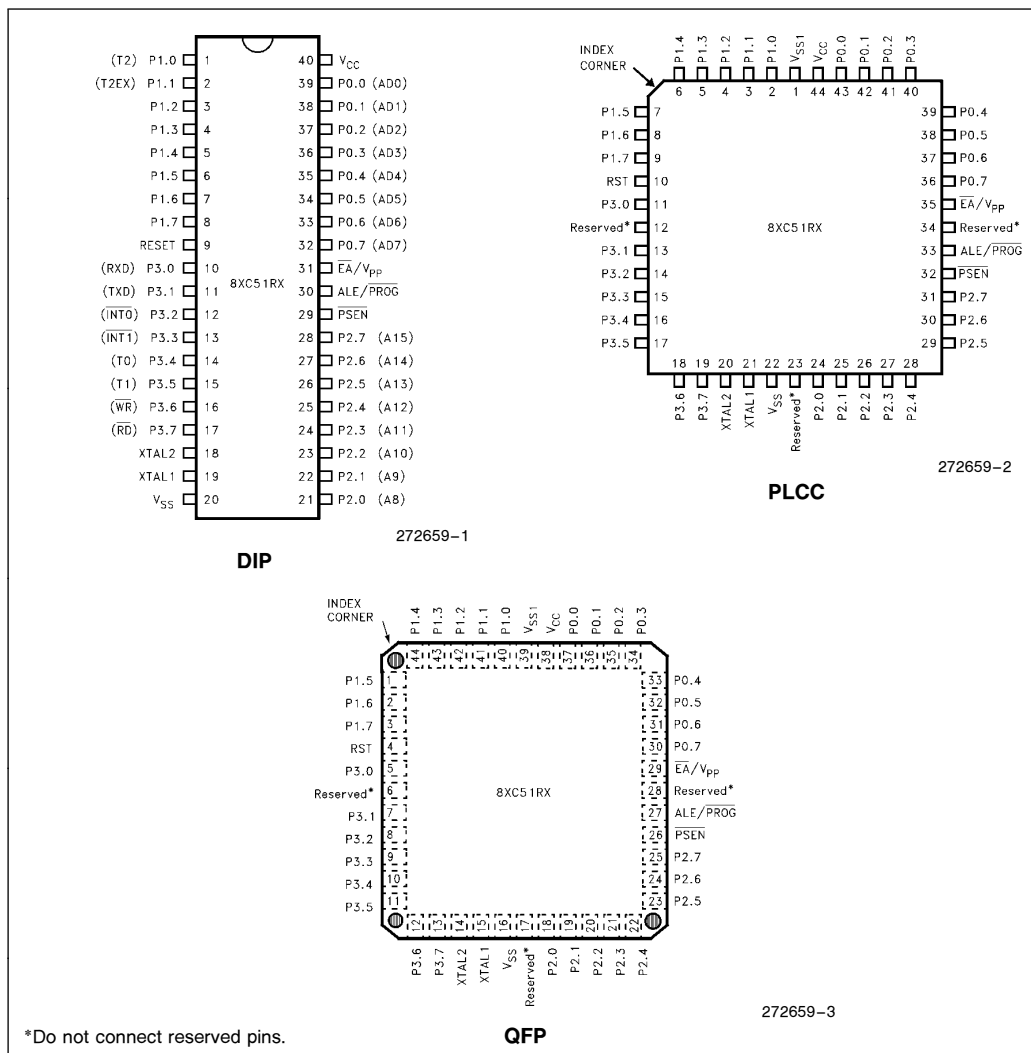
Figure 2. Pin Connections
