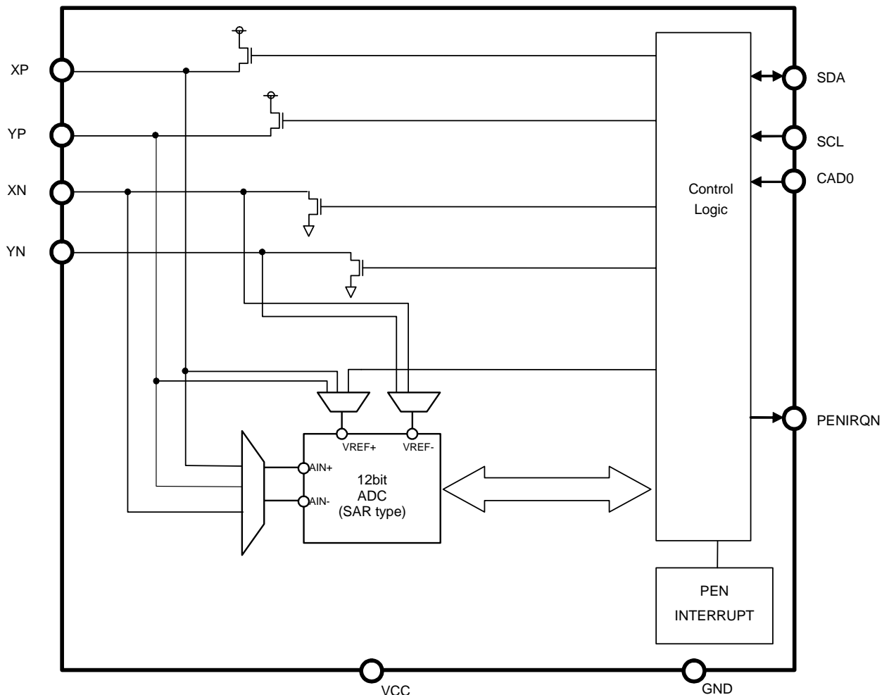
Block Diagram
