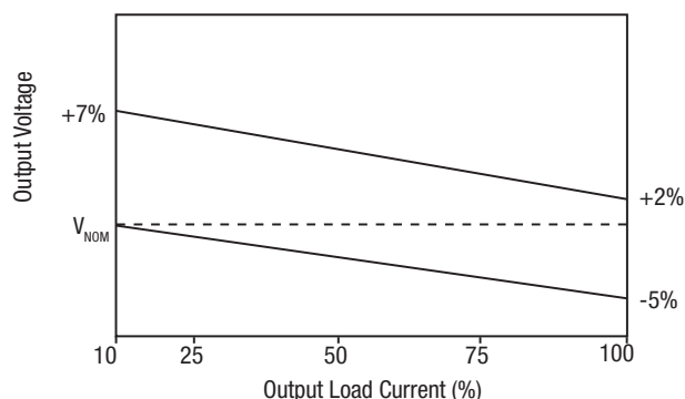
12V Output
