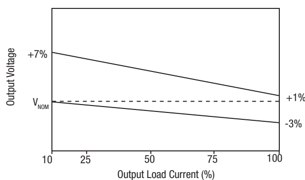
12V Output
