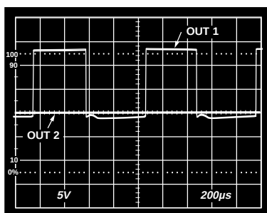
Figure 46. OUT2 Shorted to Ground, Square Wave Is OUT1, R_F = 1 \text{ k}\Omega , R_G = 222 \Omega
