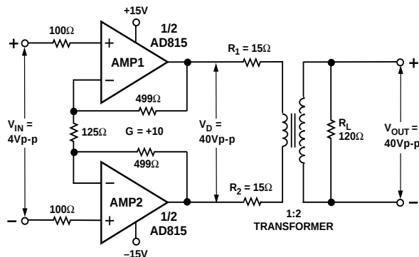
Subscriber Line Differential Driver
