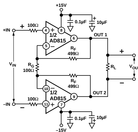
Figure 49. Fully-Differential Operation
