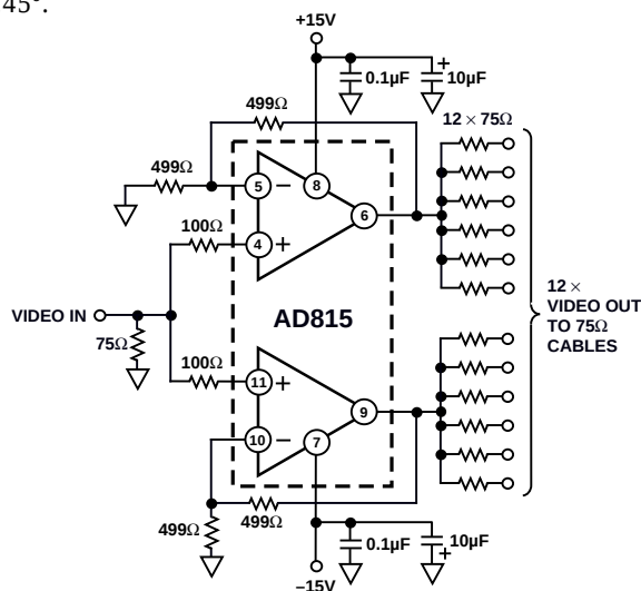
Figure 54. AD815 Video Distribution Amp Driving 12 Video Cables
