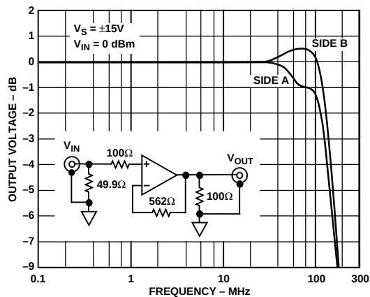
Figure 27. -3 dB Bandwidth vs. Frequency, G = +1
