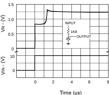
Transient Response ( I_R = 5\text{mA} )
