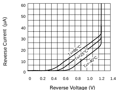
Reverse Characteristics
