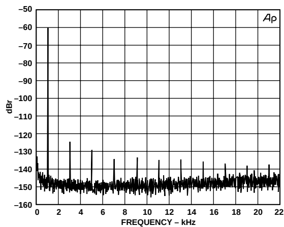
Figure 24. Dynamic Range for 1 kHz @ -60 dBFS, Triangular Dithered Input
