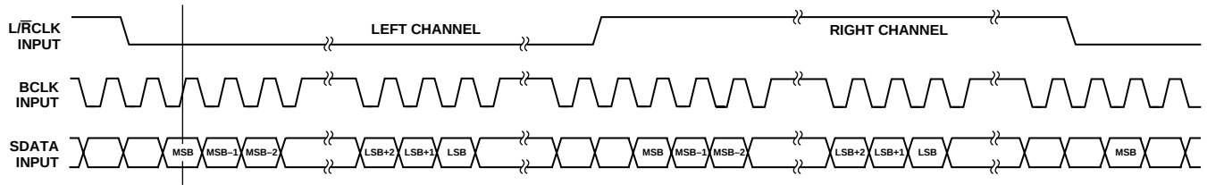
Figure 2. I2S-Justified Mode
