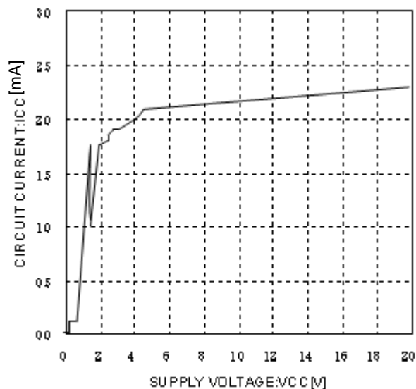
Fig.1 Circuit Current
