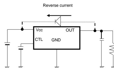
Fig.34: Bypass diode
