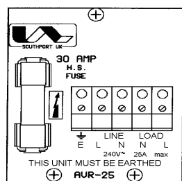
CONNECTIONS
