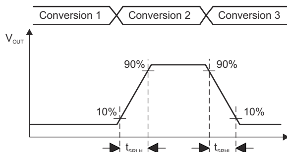
Figure 8-20. Slew Rate Testing
