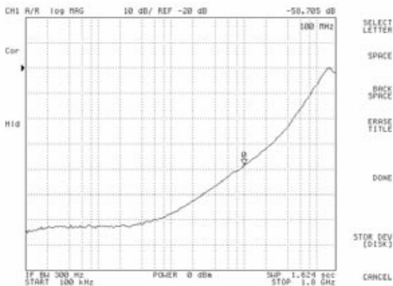
Fig 4. Off Isolation
