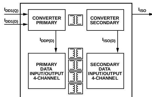
Figure 27. Power Consumption Within the ADuM5401W/ADuM5402W/ADuM5403W
