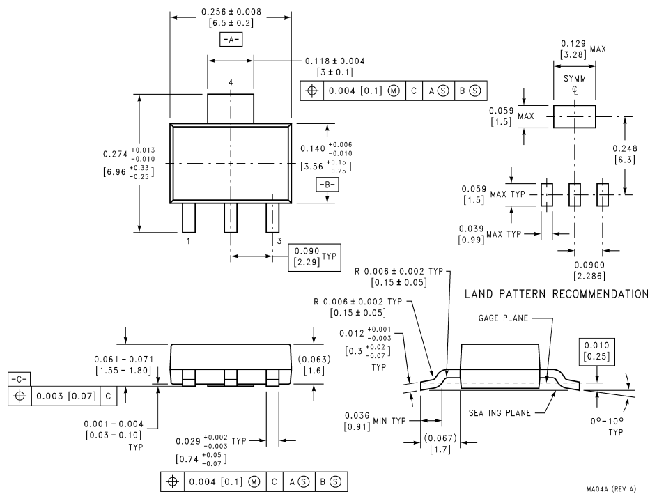
3-Lead SOT-223 Package Order Number LM317AEMP or LM317EMP NS Package Number MA04A
