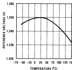
Temperature Stability
