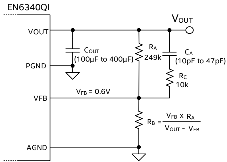
Figure 5: V_{OUT} Resistor Divider & Compensation Capacitor
