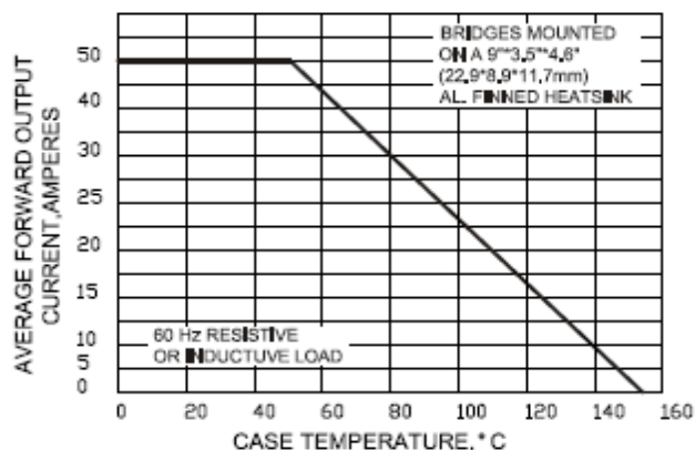
FIG.1-MAXIMUM OUTPUT RECTIFIED CURRENT
