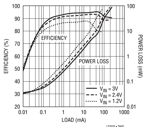
LTC3525-3.3 Efficiency and Power Loss vs Load Current
