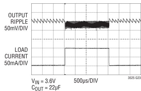
LTC3525-5 100mA Load Step Response
