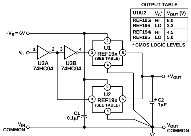
Figure 22. Switched Output Reference
