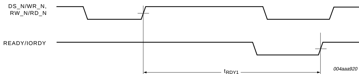
Fig 22. ISP1583 ready signal timing
