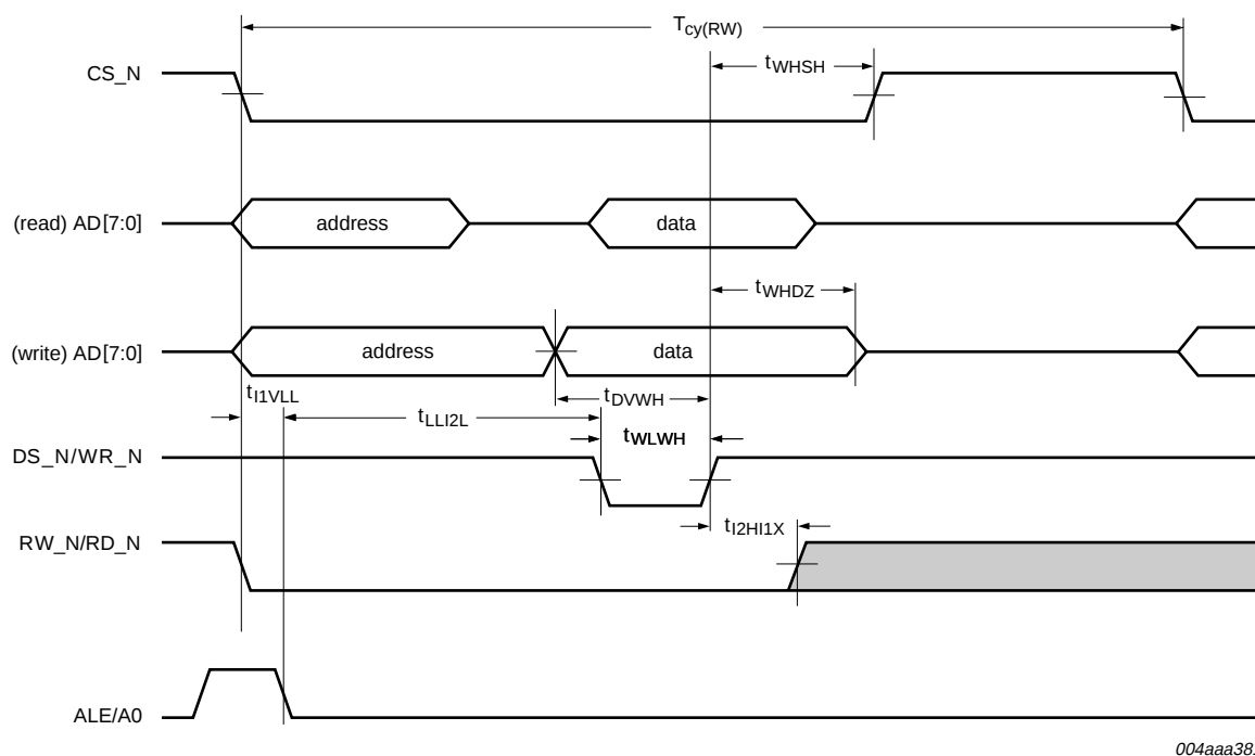
Fig 27. ISP1583 register access timing: multiplexed address/data bus (Freescale mode)
