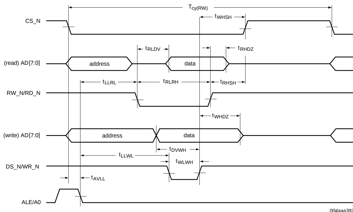
Fig 26. ISP1583 register access timing: multiplexed address/data bus (8051 mode)
