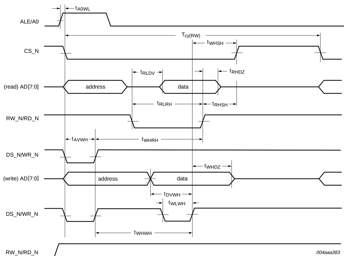
Fig 28. ISP1583 register access timing: multiplexed address/data bus (A0 function and 8051 mode)
