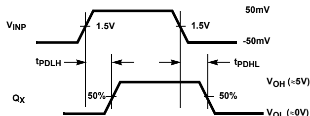
FIGURE 5. t_{PD} RECEIVER PROPAGATION DELAY MEASUREMENT POINTS
