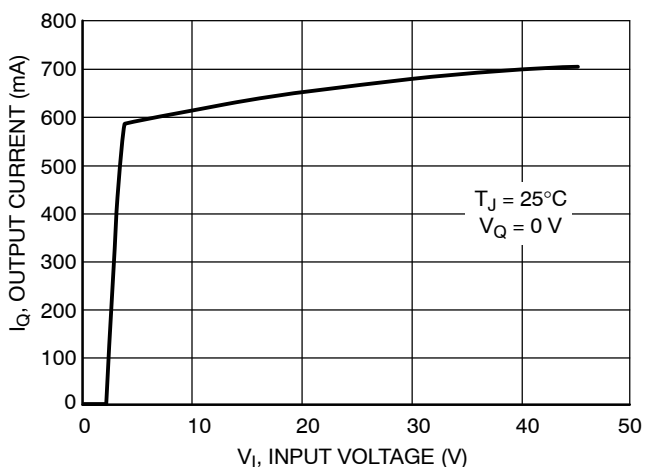
Figure 47. Maximum Output Current vs. Input Voltage, Adjustable Version
