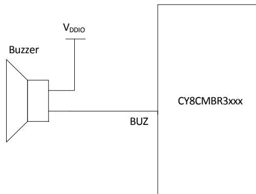
Figure 7. Buzzer Connection [4]
