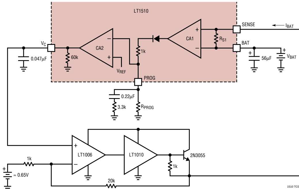
Test Circuit 1
