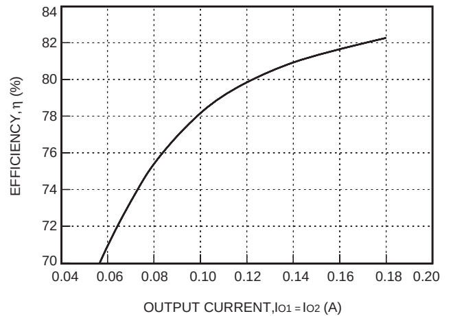
Figure 24. ME005CL Typical Converter Efficiency as a Function of Output Current with V_i = 48 V and T_A = 25 °C
