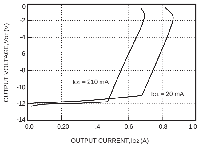
Figure 17. ME005BK Typical Output Characteristics (Vo2 vs. Io2) with Vi = 48 V and TA = 25 °C
