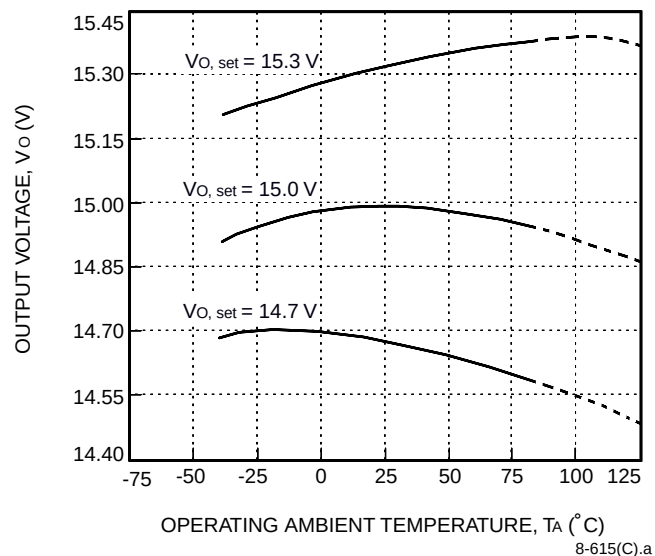
Figure 8. ME005C Typical Output Voltage Variations over Operating Ambient Temperature Range
