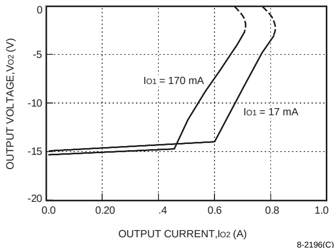
Figure 19. ME005CL Typical Output Characteristics (Vo2 vs. Io2) with Vi = 48 V and TA = 25 °C
