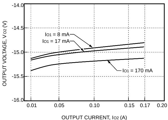
Figure 12. ME005CL Typical V_{o2} vs. I_{o2} Regulation with V_i = 48 V and T_A = 25 °C
