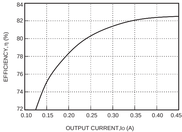
Figure 21. ME005B Typical Converter Efficiency as a Function of Output Current with V_i = 48 V and T_A = 25 °C
