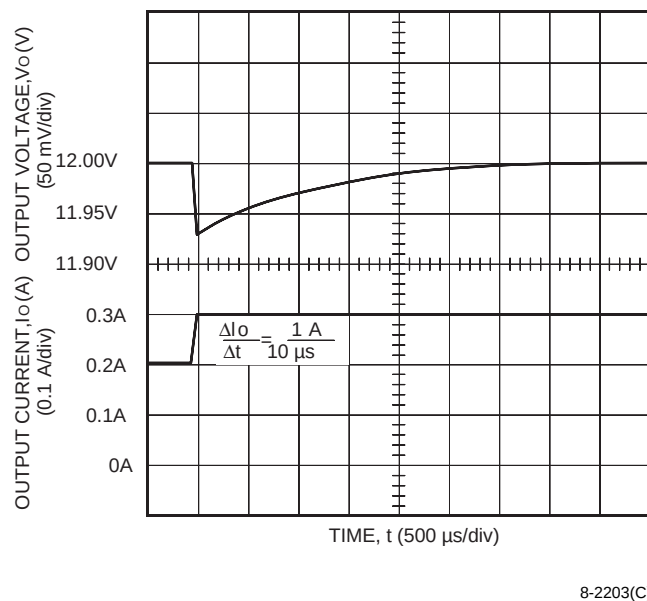
Figure 26. ME005B Typical Output Voltage Waveform for a Step Load Change from 50% to 75% of I_{o,max} with V_i = 48 V and T_A = 25 °C
