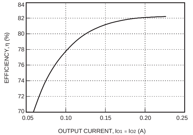
Figure 23. ME005BK Typical Converter Efficiency as a Function of Output Current with V_i = 48 V and T_A = 25 °C
