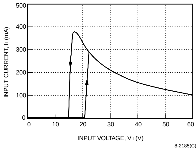
Figure 5. ME005CL Typical Input Characteristics with I_o = I_{o, \max} and T_A = 25^\circ\text{C} (Arrows Indicate Hysteresis)
