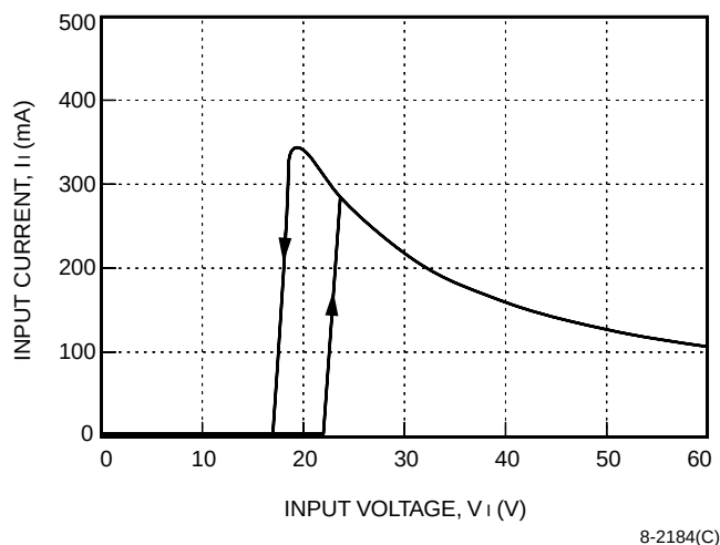
Figure 4. ME005BK Typical Input Characteristics with I_o = I_{o, \max} and T_A = 25^\circ\text{C} (Arrows Indicate Hysteresis)
