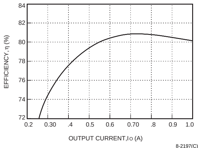
Figure 20. ME005A, N Typical Converter Efficiency as a Function of Output Current with Vi = 48 V and TA = 25 °C
