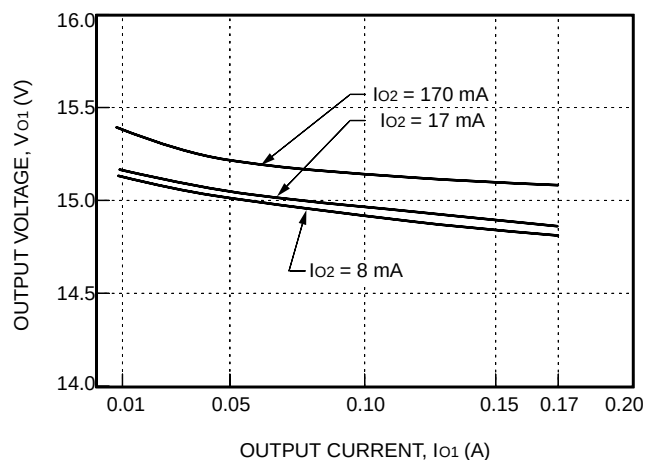
Figure 11. ME005CL Typical V_{o1} vs. I_{o1} Regulation with V_i = 48 V and T_A = 25 °C
