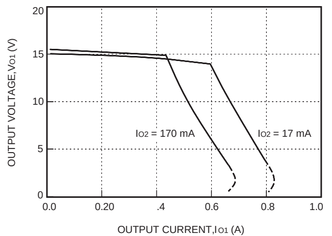
Figure 18. ME005CL Typical Output Characteristics (Vo1 vs. Io1) with Vi = 48 V and TA = 25 °C
