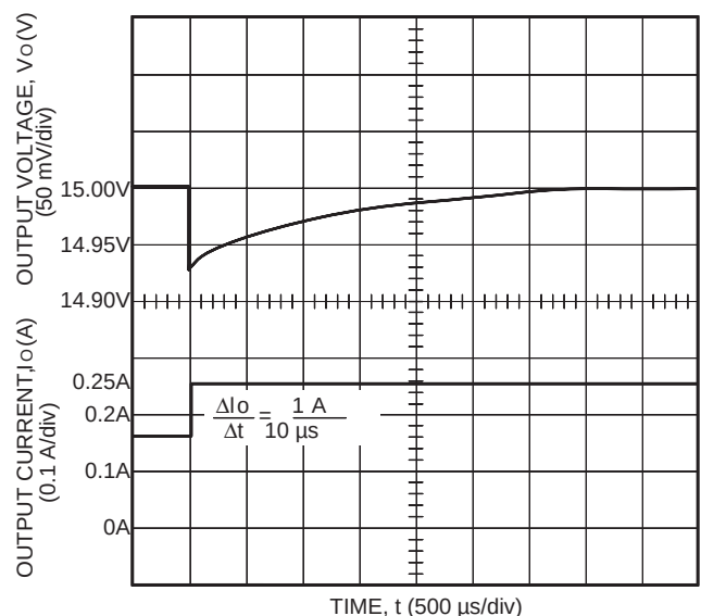
Figure 27. ME005C Typical Output Voltage Waveform for a Step Load Change from 50% to 75% of I_{o,max} with V_i = 48 V and T_A = 25 °C
