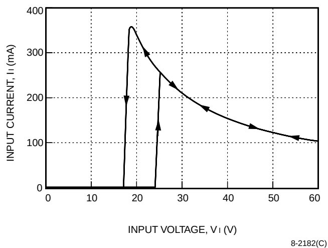
Figure 2. ME005B Typical Input Characteristics with I_o = I_{o, \max} and T_A = 25^\circ\text{C} (Arrows Indicate Hysteresis)
