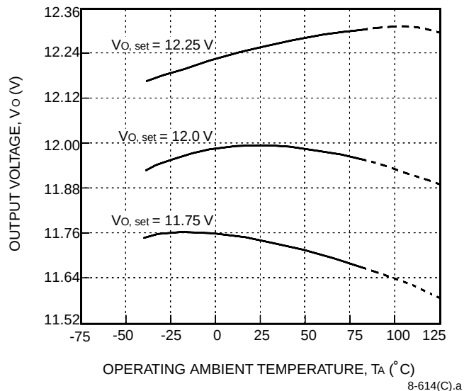
Figure 7. ME005B Typical Output Voltage Variations over Operating Ambient Temperature Range
