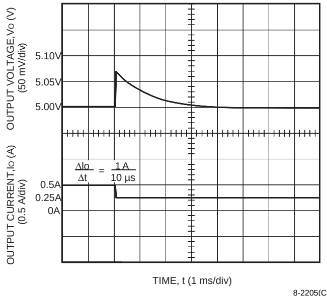
Figure 28. ME005A Typical Output Voltage Waveform for a Step Load Change from 50% to 25% of I_{o,max} with V_i = 48 V and T_A = 25 °C (ME005N Waveform Is Similar, but with 5.2 V Steady-State.)
