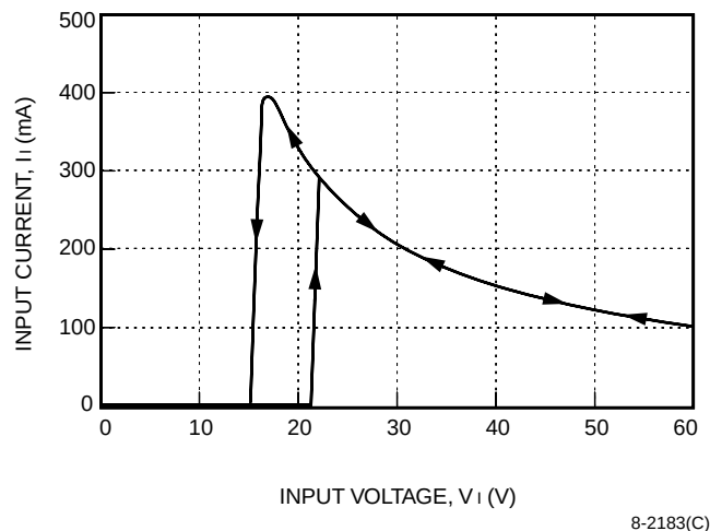
Figure 3. ME005C Typical Input Characteristics with I_o = I_{o, \max} and T_A = 25^\circ\text{C} (Arrows Indicate Hysteresis)
