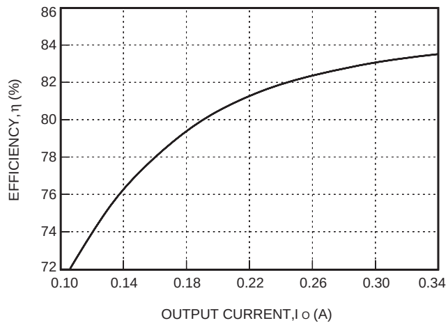
Figure 22. ME005C Typical Converter Efficiency as a Function of Output Current with V_i = 48 V and T_A = 25 °C
