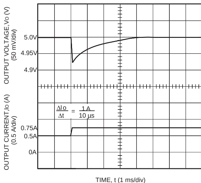
Figure 25. ME005A Typical Output Voltage Waveform for a Step Load Change from 50% to 75% of I_{o,max} with V_i = 48 V and T_A = 25 °C (ME005N Waveform Is Similar, but with 5.2 V Steady-State.)
