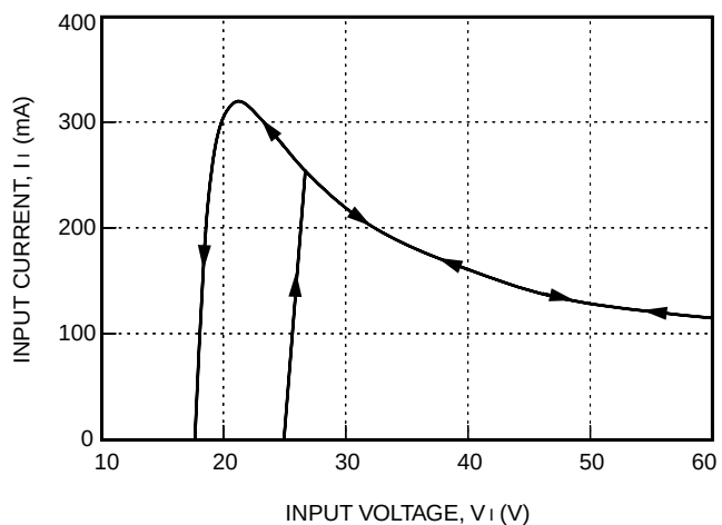
Figure 1. ME005A, N Typical Input Characteristics with I_o = I_{o, \max} and T_A = 25^\circ\text{C} (Arrows Indicate Hysteresis)
